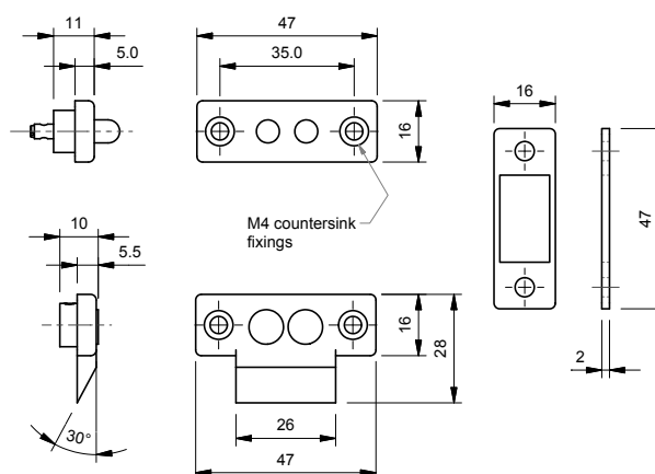
Fig.9 Door proving contact set
