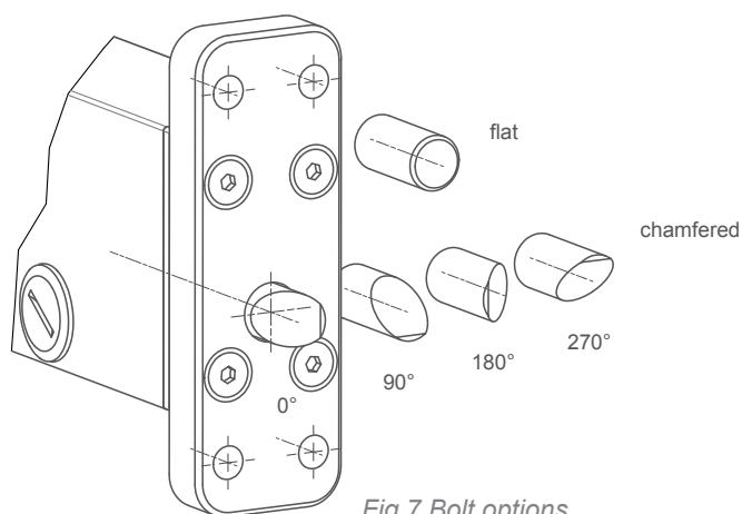
Fig.7 Bolt options
