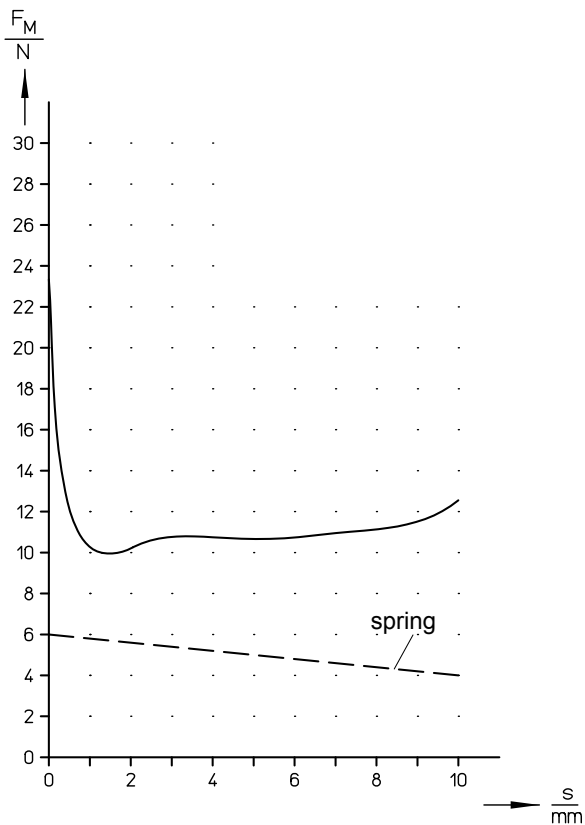
Fig. 10: Force vs. stroke characteristic and return spring for G SC X 045 N43 A01
