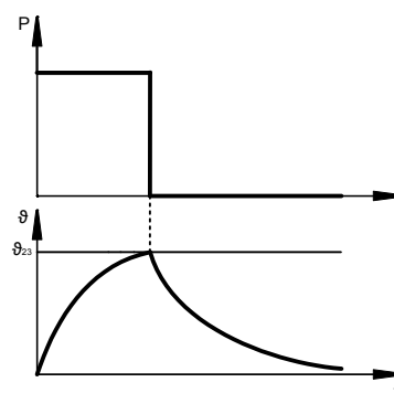
Fig. 27: Temperature curve short-time duty
