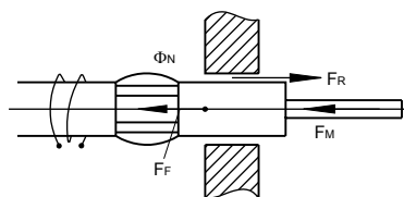
Fig. 17: Magnetic force
