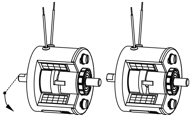
Fig. 10: Cross section ON/OFF rotary solenoid
