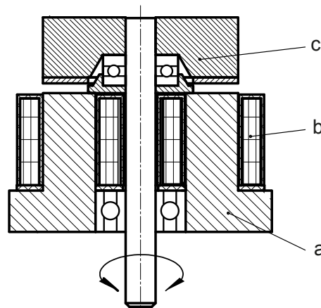
Fig. 13: Principle proportional rotary solenoid G DR
