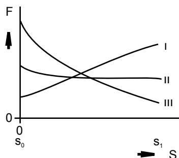
Fig. 20: Types of the magnetic force vs. stroke characteristic
