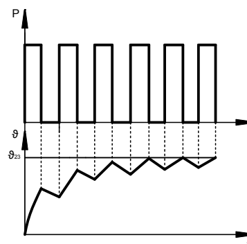
Fig. 26: Temperature curve intermittent operation
