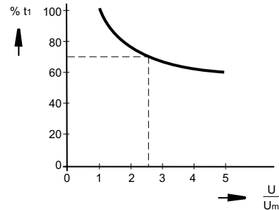
Fig. 31: Reduction attraction time depending on the voltage quotient
