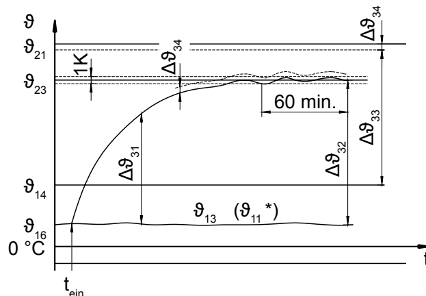
Fig. 38: Temperatures at solenoids
